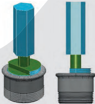
Figure 1 - Minimum CP
